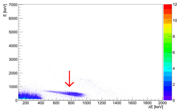
Figure 3. \Delta E -E coincidences matrix for events detected in the telescope. The red arrow points to the region of protons emitted in the {}^7\text{Be}(n,p){}^7\text{Li} reaction.
