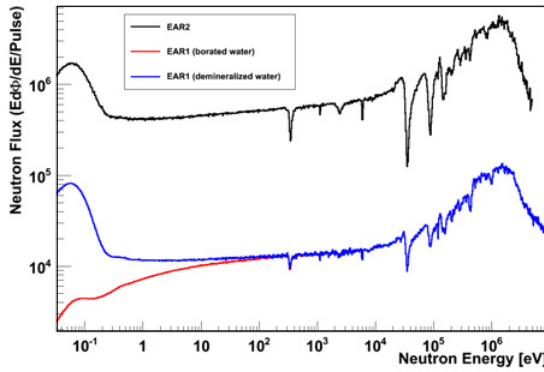
Figure 1. n_TOF neutron flux at EAR1 with normal (blue) and borated (red) water as moderator compared with the neutron flux at EAR2 (black) [8].
