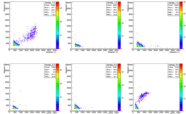
Figure 2. Scatter plot for signal amplitudes in all possible pairs of detectors of the stack. Top left and bottom right plot refer to pairs hosting the ^7\text{Be} sample, they clearly shows the expected back-to-back coincidences not present in uncorrelated pairs of silicon.
